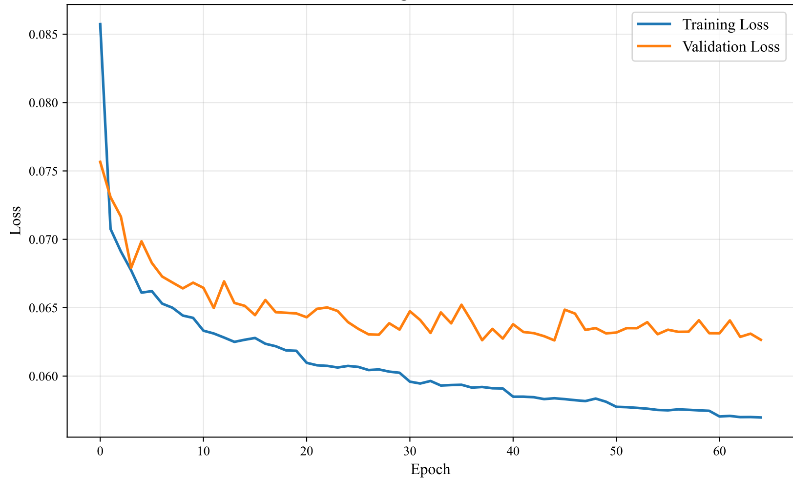
Bi-TSENet Training & Validation Loss - data8
